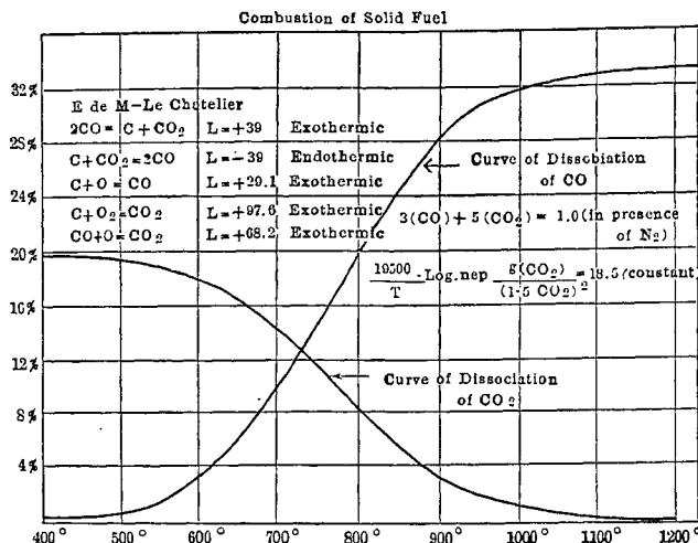
FIG. 180.—Equilibrium Curves of CO and CO 2 in the Presence of Nitrogen. In the combustion of solid fuel the reaction occurs with a rising temperature \text{CO}_2 + \text{C} = 2\text{CO} when the temperature drops, particularly in the presence of iron oxide the reaction reverses, 2\text{CO} = \text{CO}_2 + \text{C} .
