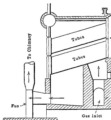
FIG. 157.—Proposed Setting of Marine Type of Waste Heat Boiler.
