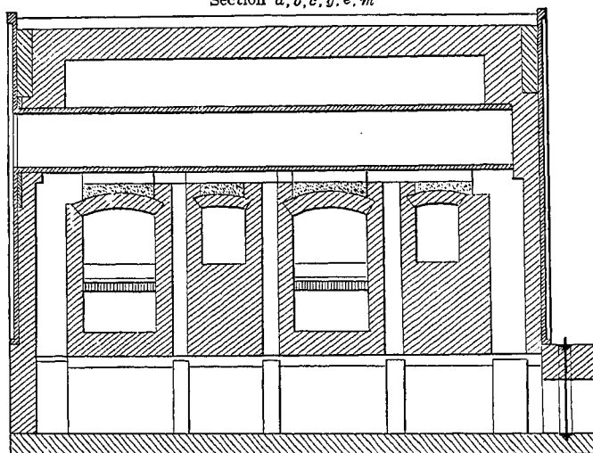
FIG. 134.—Longitudinal Section.
