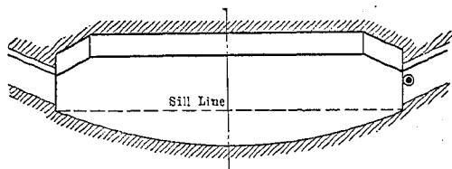
FIG. 149.—Heating Chamber with Raised Straight Roof.
