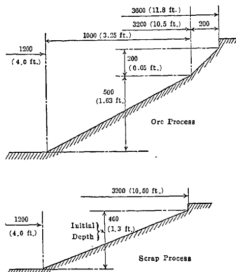
FIG. 142.—Sections Showing Profile of Hearth Slope According to Professor Groume-Grjimallo.
