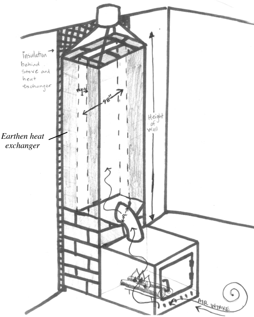
An example of an earthen heat exchanger
